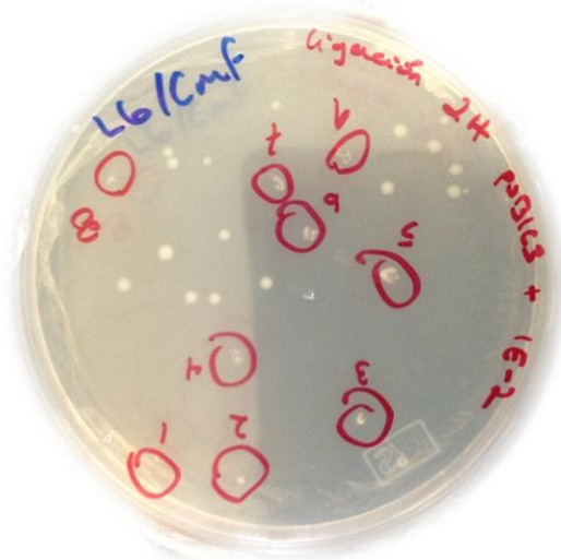
Big colonies 😊
